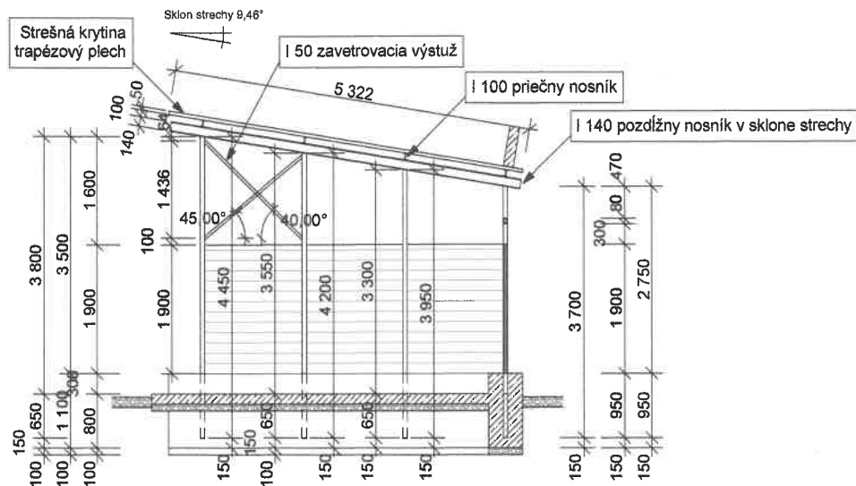
SO 10.2 Rez priecny C/C
