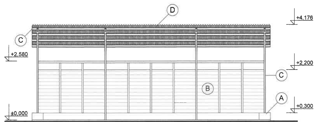
SO 10.2 Rez priecny C/C
